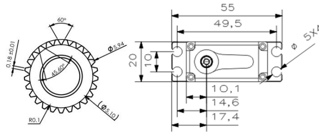
25T 6mm Output Shaft Spline
